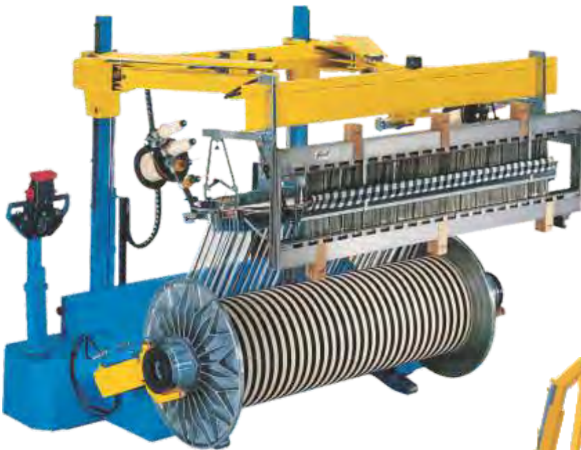
Completely Motorised Quick Style Change (QSC) Trolley
