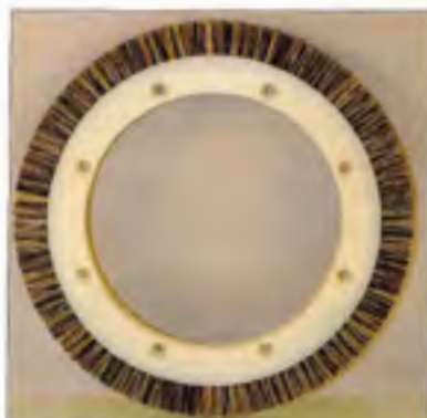
Reggianni brushing ring 240 mm diameter
